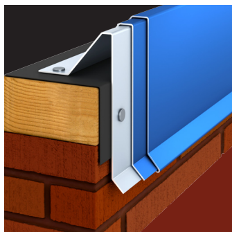
Gravel Stop
